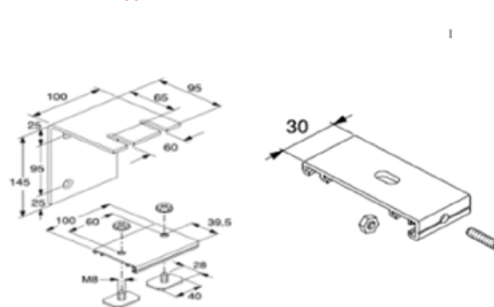
Wall brackets support
