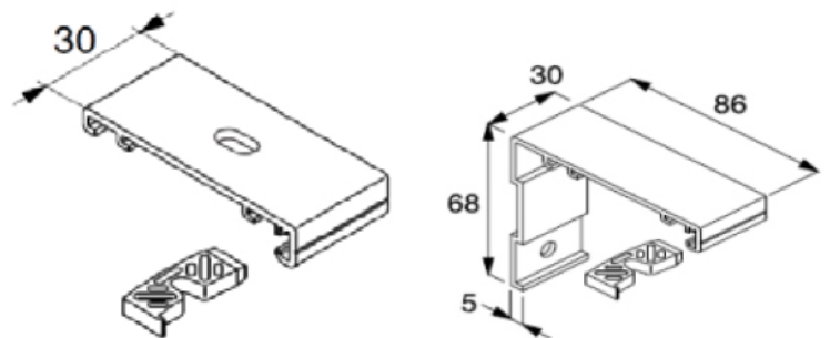
Bracket Detail
